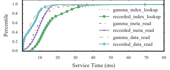
Figure 5. The results of fitting the disk service times
